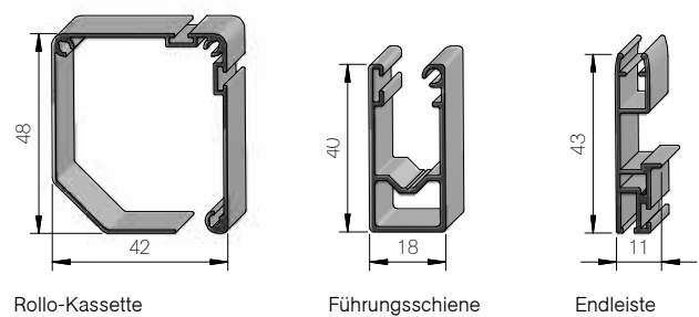
Rollo-Kassette
