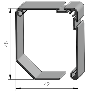
Rollo-Kassette
