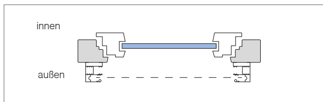
Rollo-Kassette
